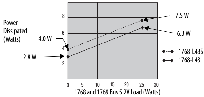
Figure 10 - 1768-L43 and 1768-L43S Power Dissipation
