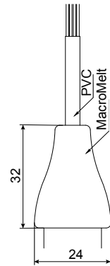
LBFS-x2xxx.x Cable outlet
