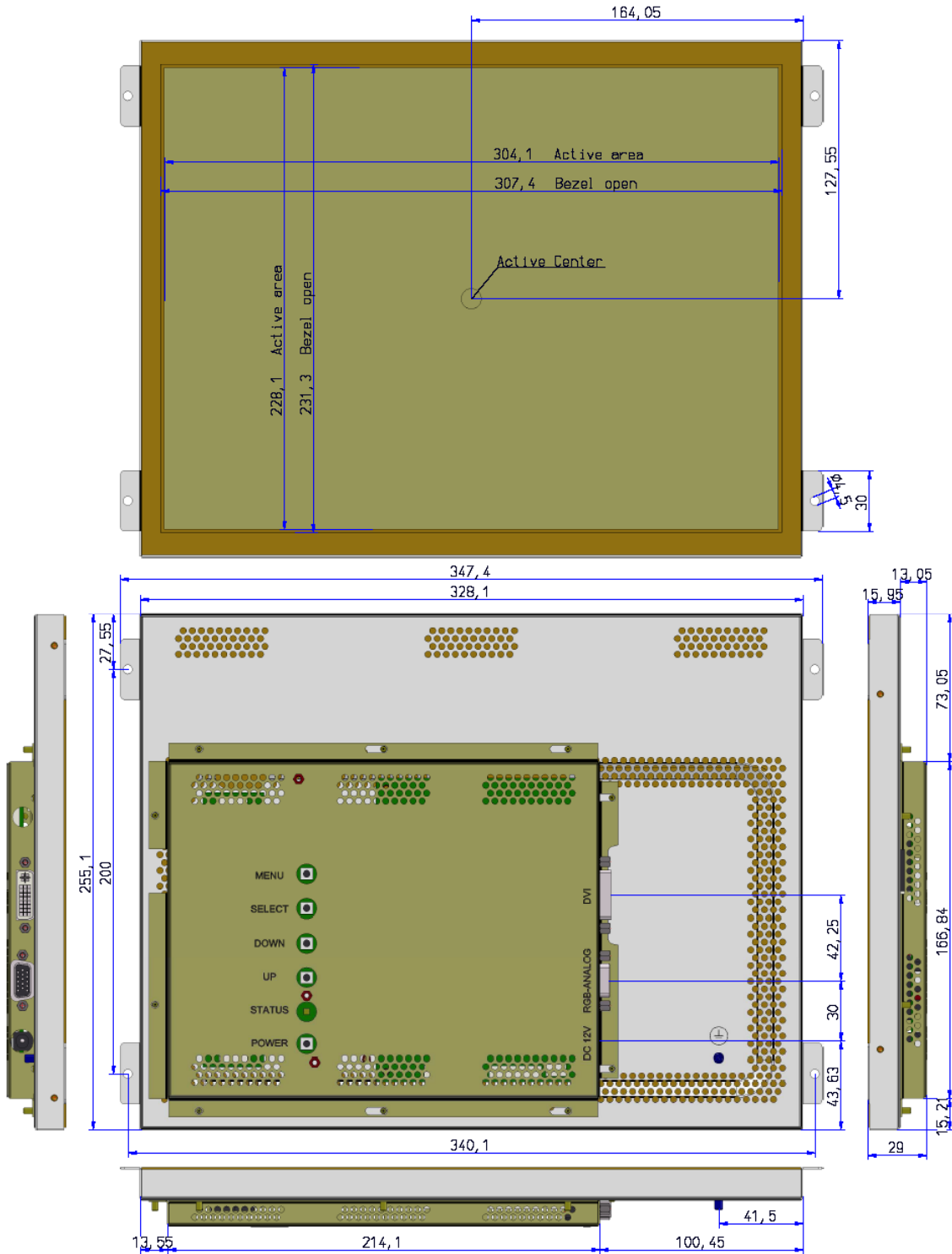
Figure 1: Mechanical Outlines
