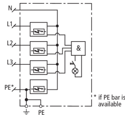
Basic circuit diagram DSH ZP B TT 255
