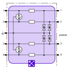
Basic circuit diagram BXT ML4 BE 12
