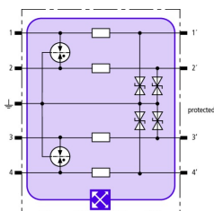
Basic circuit diagram BXT ML4 BE 180
