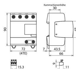
Dimension drawing DV M2 TNS 255 FM
