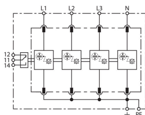
Basic circuit diagram DV M2 TNS 255 FM
