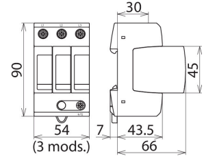
Dimension drawing DG MU 3PD 480 3W+G
