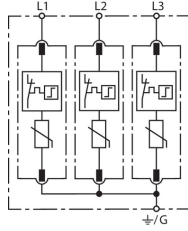
Basic circuit diagram DG MU 3PD 480 3W+G
