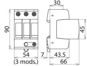
Dimension drawing DG MU 3PY 480 3W+G
