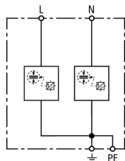
Basic circuit diagram DSH TN 255
