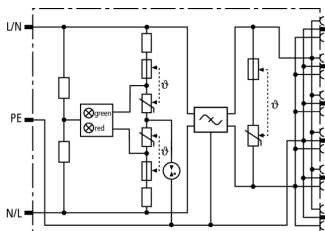
Basic circuit diagram SFL PRO 6X 19"
