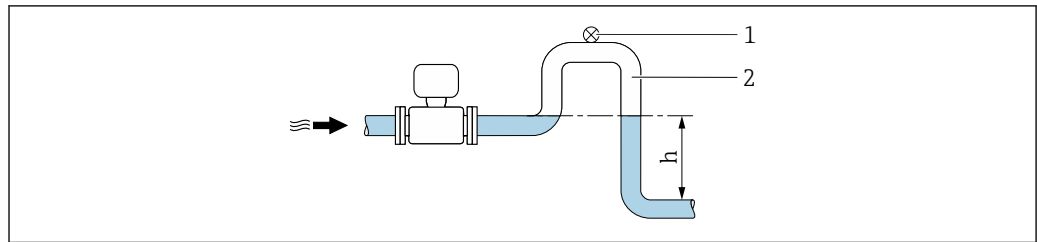
27 Installation in a down pipe
