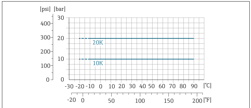
36 Process connection material: stainless steel (-20 °C (-4 °F)); carbon steel (-10 °C (14 °F))
