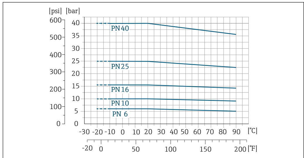
33 Process connection material: stainless steel (-20 °C (-4 °F)); carbon steel (-10 °C (14 °F))
