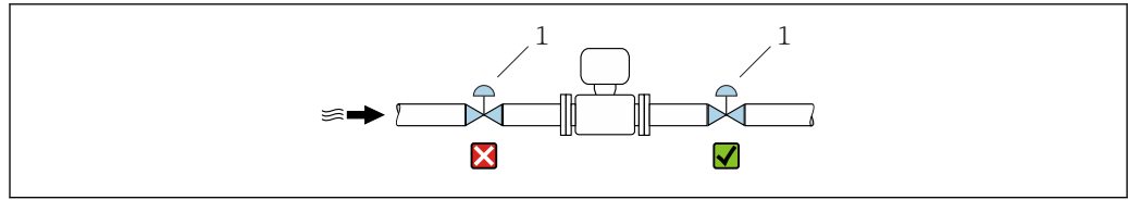
26 Installation of the sensor after a control valve is not recommended
