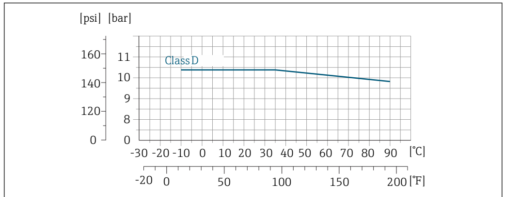
37 Process connection material: carbon steel
