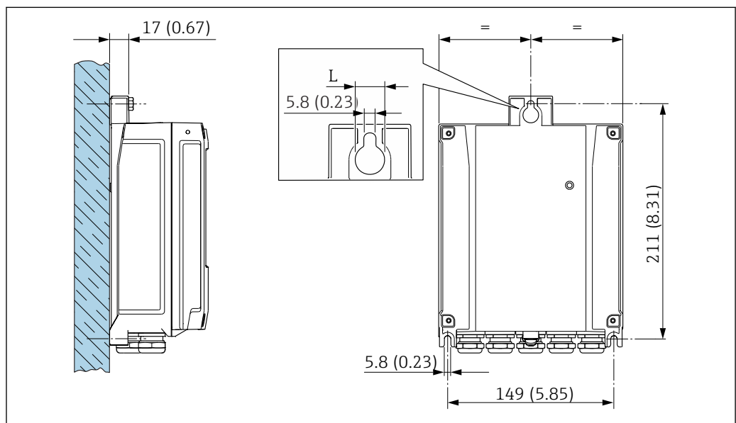
30 Engineering unit mm (in)
