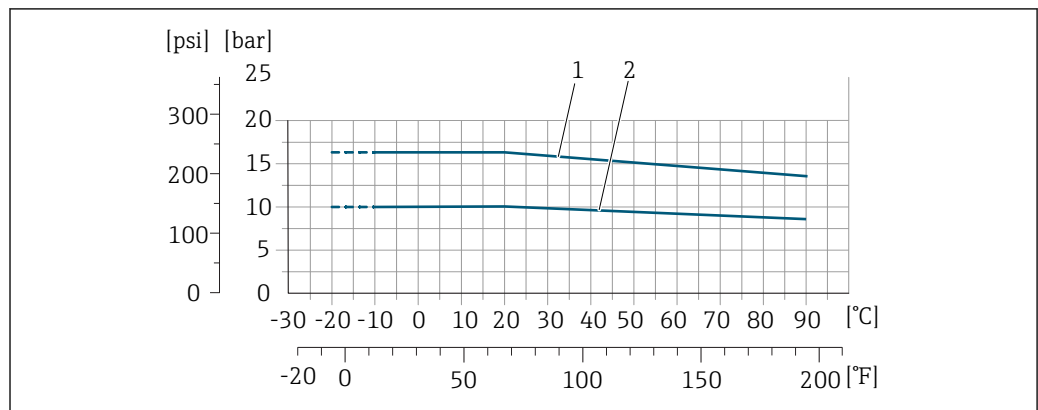
40 Process connection material: stainless steel (-20 °C (-4 °F)); carbon steel (-10 °C (14 °F))
