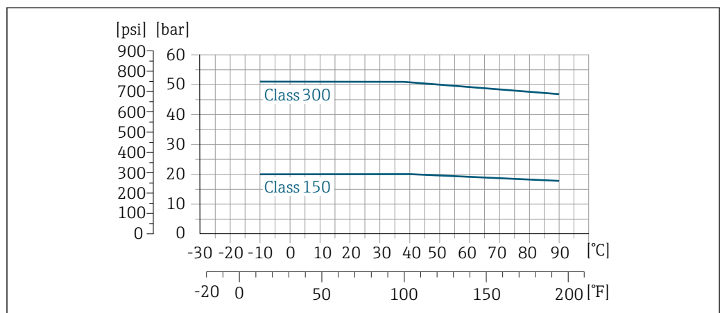
35 Process connection material: carbon steel
