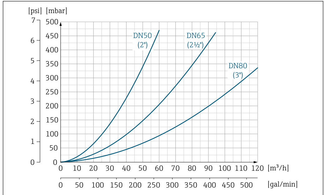
41 Pressure loss DN 50 to 80 (2 to 3") for order code for "Design", option C "fixed flange, without inlet/outlet runs"
