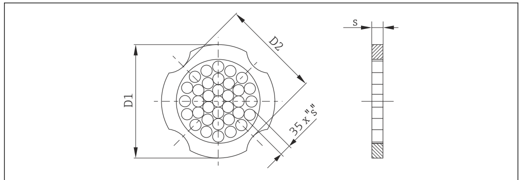
Flow conditioner according to EN 1092-1 (DIN 2501): PN 10/16 Order code for "Accessory enclosed", option PF
