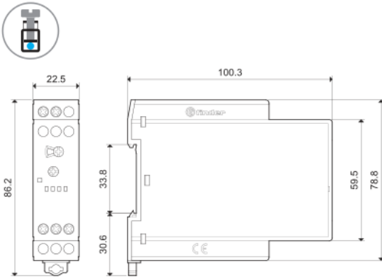
83.11 Screw terminal
