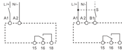
Wiring diagram (without control signal) Wiring diagram (with control signal)
