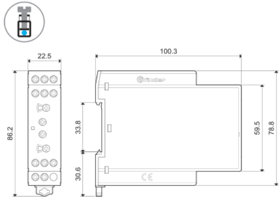
83.02 Screw terminal
