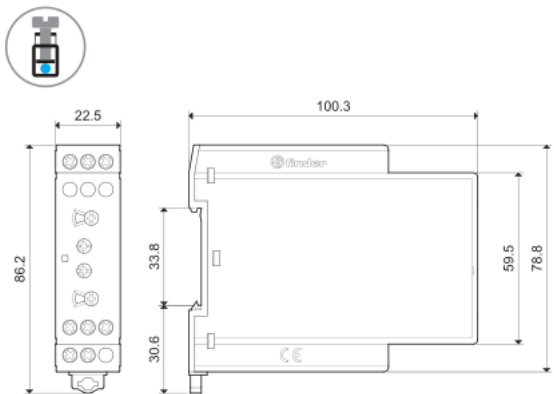
83.91 Screw terminal
