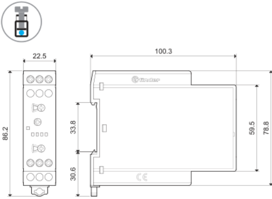
83.01 Screw terminal
