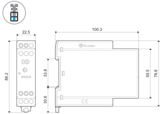
83.21 Screw terminal
