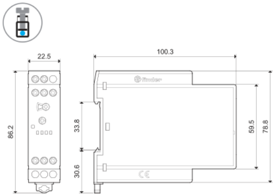
83.62 Screw terminal
