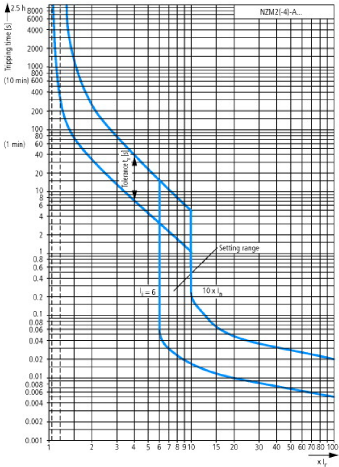
Characteristic curves
