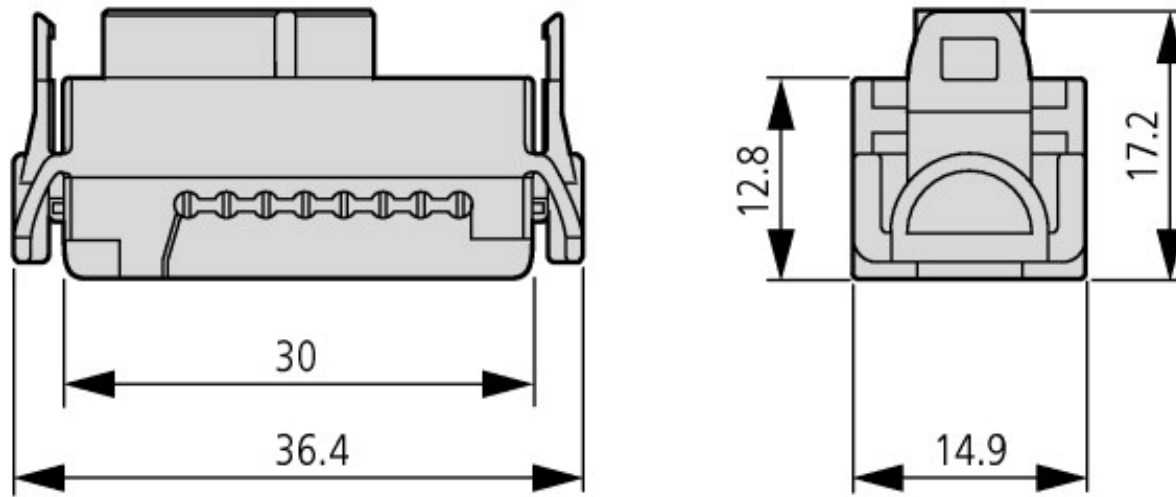
External device plugs
