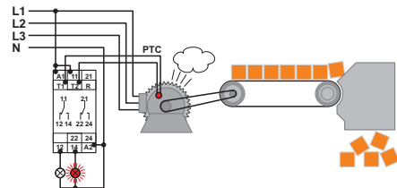
Shutdown and message in case of overload
