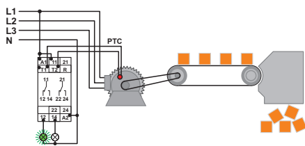
Monitoring of motor winding temperatures
