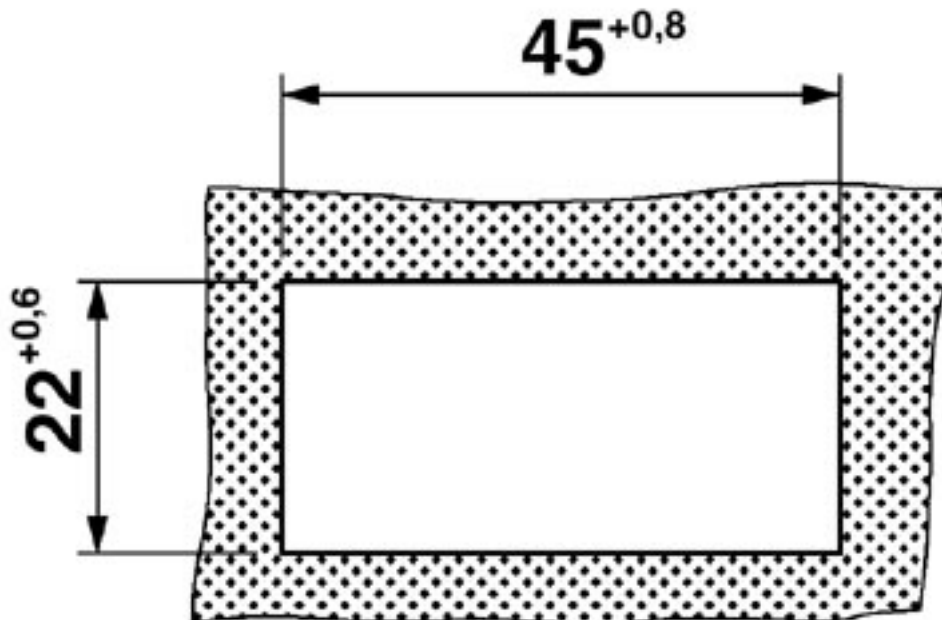
Dimensioned drawing
