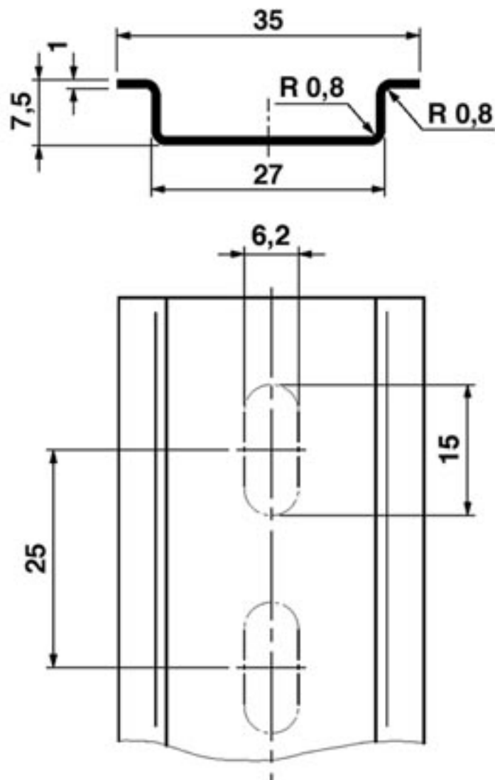
Dimensioned drawing
