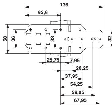
Dimensional drawing
