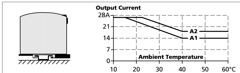
Fig. 26-12 Mounting Orientation C (Table-top mounting)
