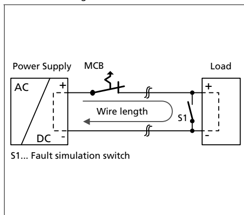
Fig. 26-9 Test circuit
