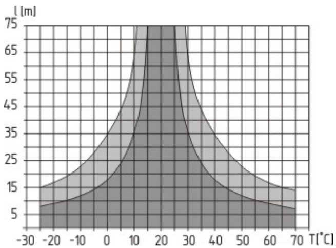
Characteristic curve
