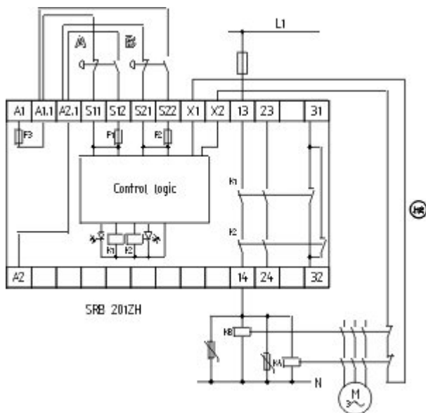
Wiring example
