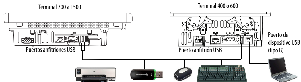
Figura 14 – Puertos USB
