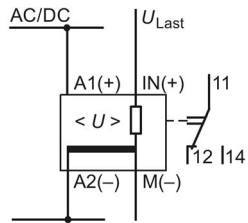
Figura 10-1 3UG4631-.AA30/3UG4632-.AA30
