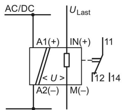
Figura 10-2 3UG4631-.AW30/3UG4632-.AW30
