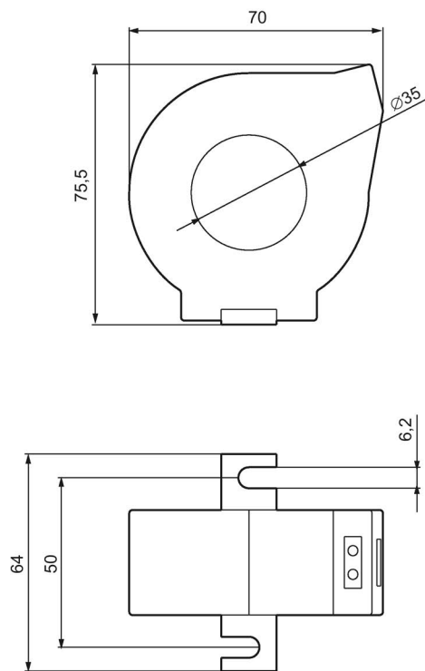
Figura 13-9 3UL2302-1A
